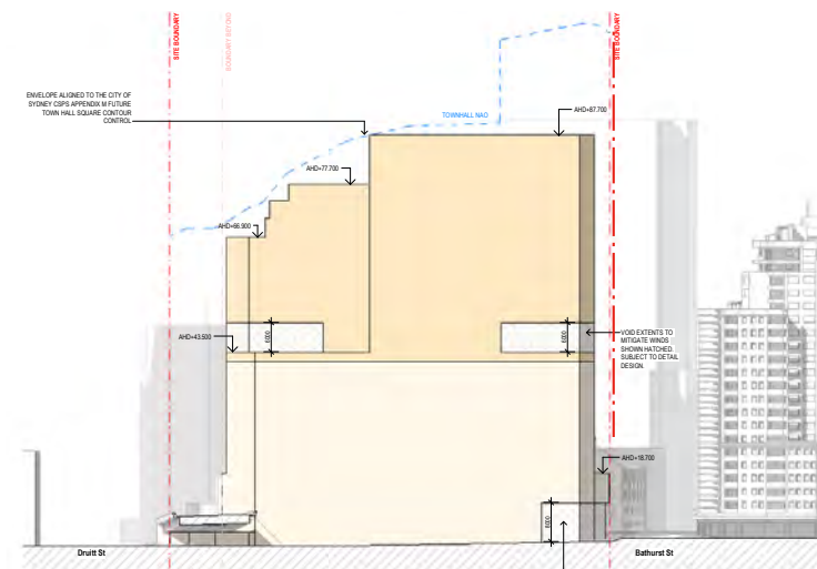
WEST ELEVATION
