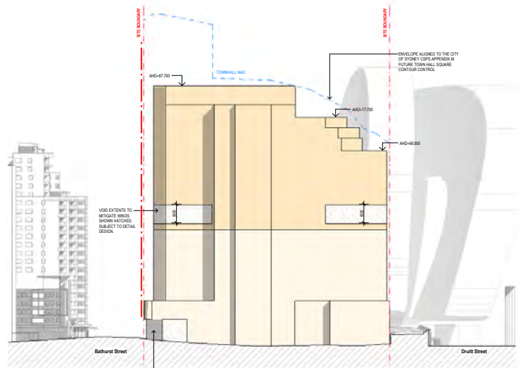
EAST ELEVATION
